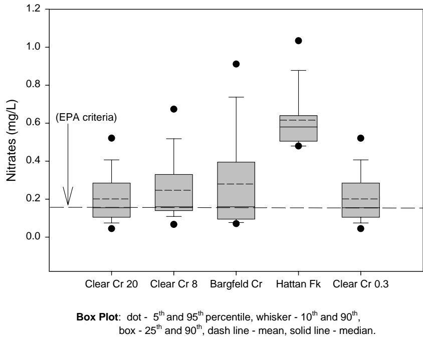
Figure 7-4: Nitrates measured in Clear Creek, 2000 and 2001.
