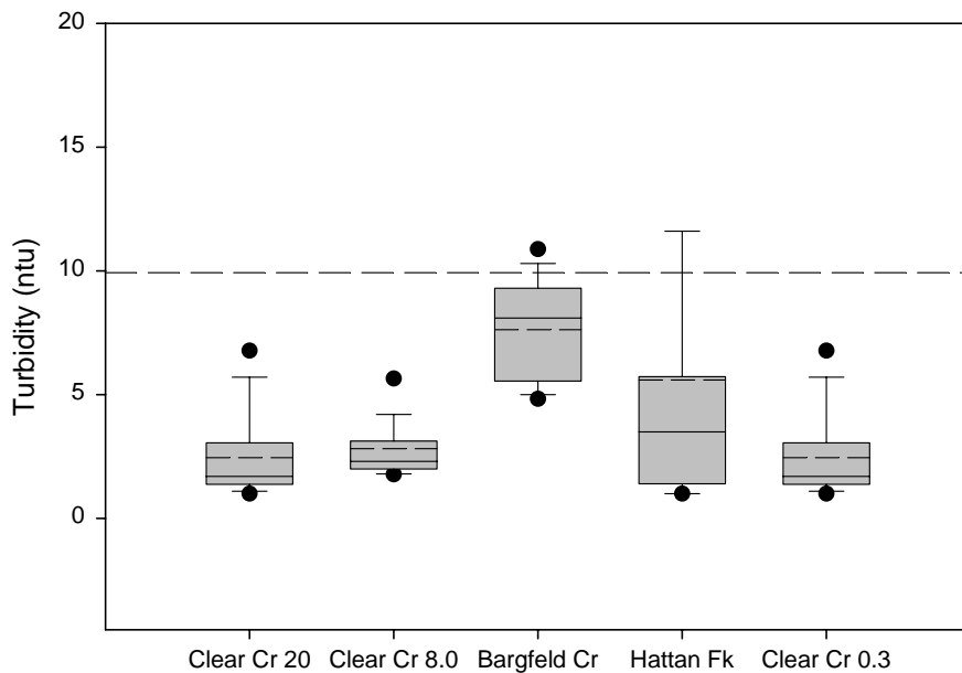
Figure 7-8: Turbidity (NTU) measured in Clear Creek, 2001.
